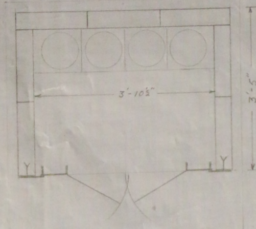
GENERAL ARRANGEMENT CONCRETE BLOCK HOUSE MENGEARY POINT LIGHT
